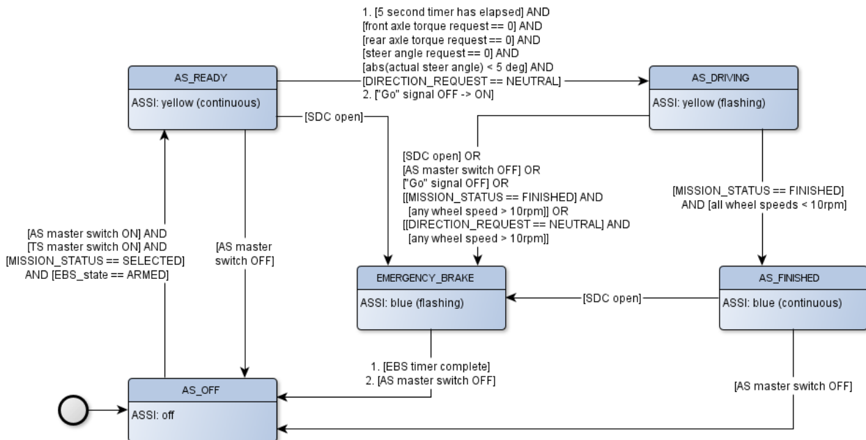
Figure 1: Autonomous driving state machine
